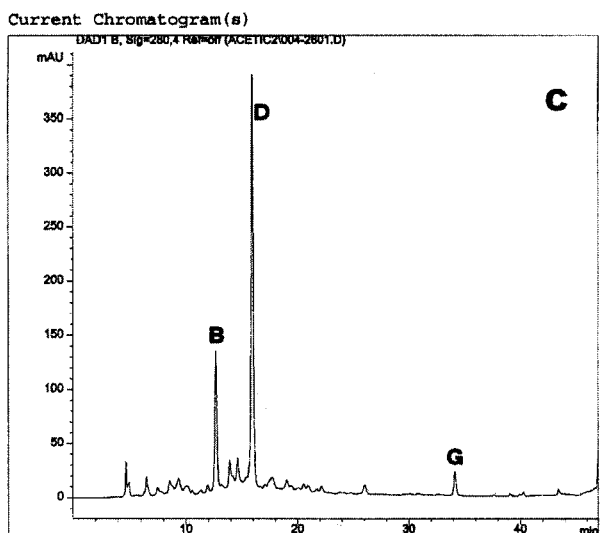
Figure 2. HPLC chromatograms of pomegranate phenolics recorded at 280 nm. (Panel A) Juice 1 directly obtained from arils; (Panel B) Commercial single-strength juice 3 (extracted from whole pomegranates); (Panel C) Husk water extract (1 g homogenized in 100 mL water). A = galloylglucose; B = punicalagin isomer; C = hydrolyzable tannin; D = punicalagin isomer; E = delphinidin 3-glucoside; F = cyanidin 3-glucoside; G = ellagic acid.
