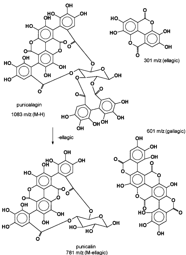
Figure 4. HPLC-MS (electrospray ionization) fragmentation of compounds B and D (punicalagin isomers). The fragments punicalin (781 m/z ), gallagic (601 m/z ) and ellagic acid (301 m/z ) are observed.
