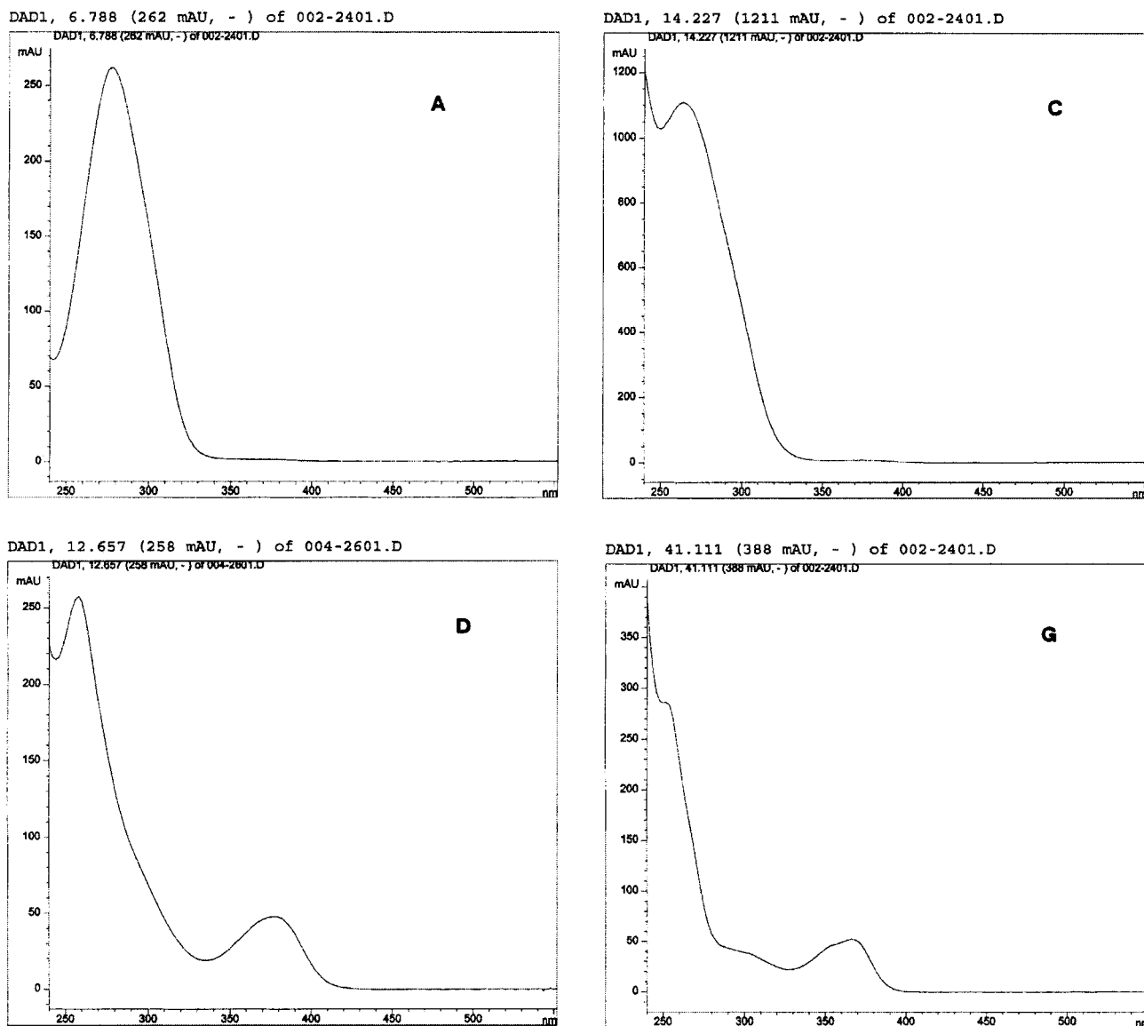
Figure 3. UV spectra of pomegranate juice characteristic compounds. A = galloylglucose; C = hydrolyzable tannin; D = punicalagin; G = ellagic acid.
