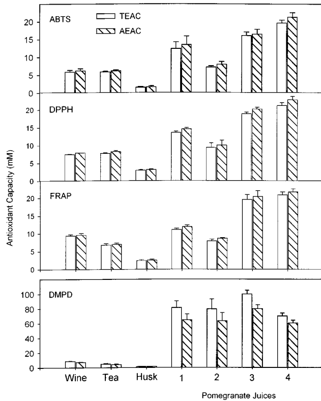
Figure 1. Antioxidant capacity of pomegranate juices compared to those of red wine, green tea and a water extract of pomegranate fruit husk (rind) evaluated by the ABTS, DPPH, FRAP, and DMPD methods. The values represent the Trolox equivalent antioxidant capacity (TEAC) and ascorbic acid equivalent antioxidant capacity (AEAC). The antioxidant capacity of the different food products is equivalent to those of Trolox and ascorbic acid solutions with the indicated concentrations (mM).
